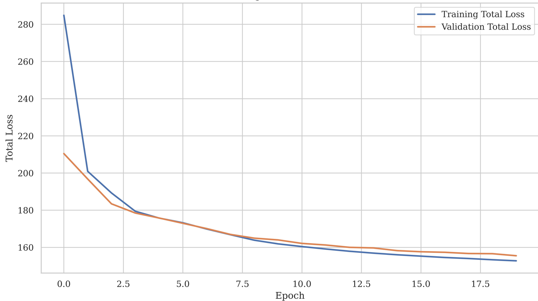
VAE Training and Validation Total Loss
